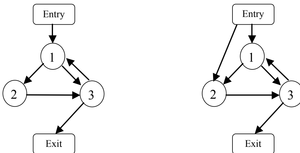
dyninstAPI (a) An example of natural loop
